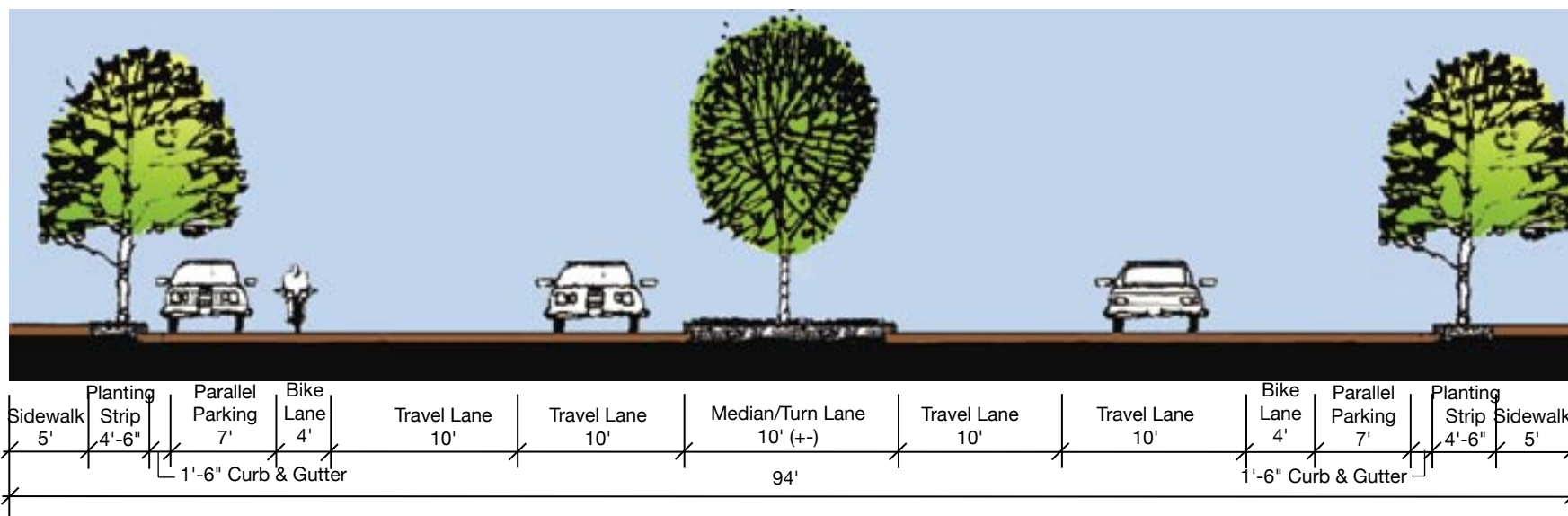
Street Section B - 90' Cross Section (Between Beall Street and Durston Road)
