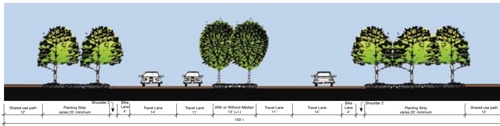
Street Section C - 150' + Section
