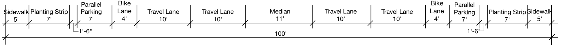
Street Section B - 100' Cross Section (Between Durston Road and I-90)
